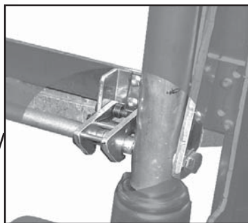
Latch keeps 4th wheel up when not in use.
