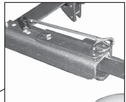
Latch and pin system keeps the 4th wheel extended (2002-E37L)
