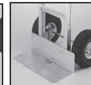
C17, C13 18" x 7.5" Front Mount Extruded Aluminum C17- w/o Cutouts C13- w/ Cutouts
