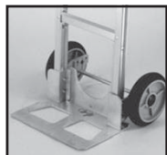
C1, C19 14" x 7.5" Recessed Heel C1 w/ Cutouts C19 w/o Cutouts Extruded Aluminum
